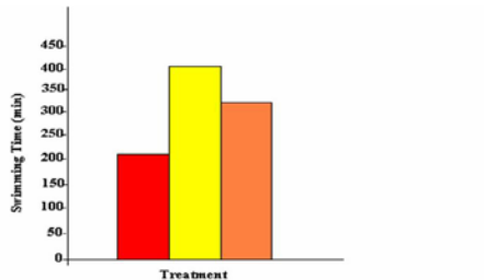
Figure 1: Effect of ethanolic extract of Withania somnifera and aqueous root powder of Panax ginseng on swimming performance in mice.
