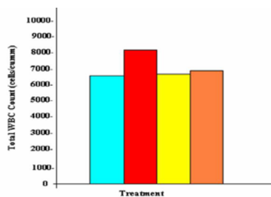
Figure 2: Effect of ethanolic extract of Withania somnifera and aqueous root powder of Panax ginseng on cold restraint stress induced changes in total WBC count in mice.
