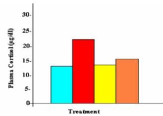
Figure 4: Effect of ethanolic extract of Withania somnifera and aqueous root powder of Panax ginseng on cold restraint stress induced changes in plasma cortisol level in mice.
